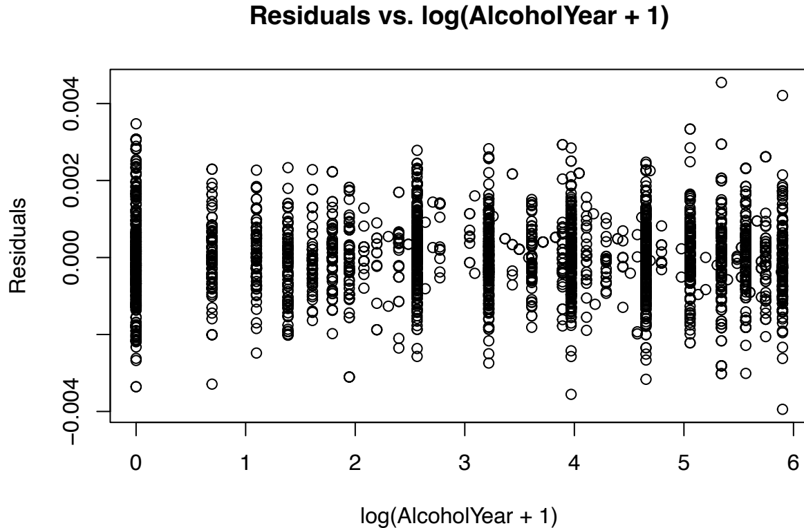
Figure 5: Residuals vs. \log(\text{AlcoholYear} + 1) in the final model
