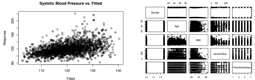
Figure 1: Response vs. Fitted plot (left) and pairwise predictor plot (right) for the preliminary model
