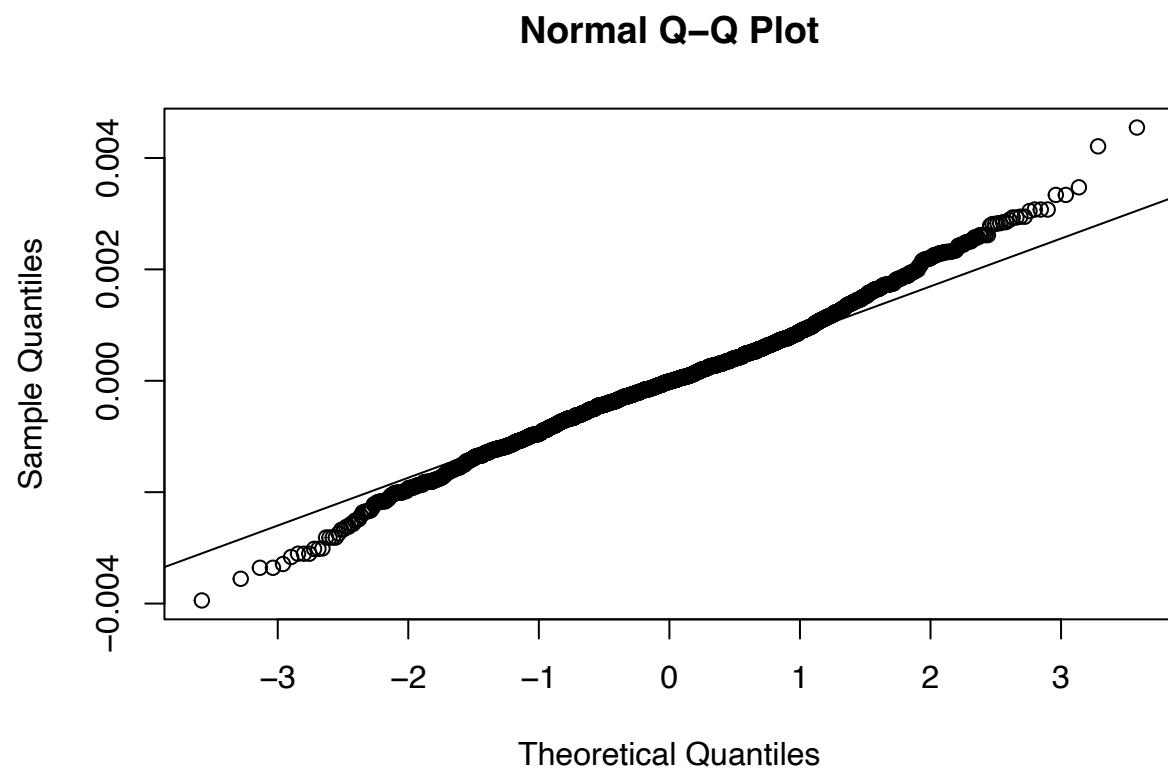
Figure 8: Q-Q plot for the final model
