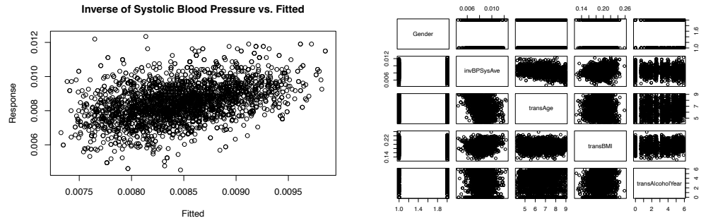
Figure 6: Condition 1 and 2 for the final model
