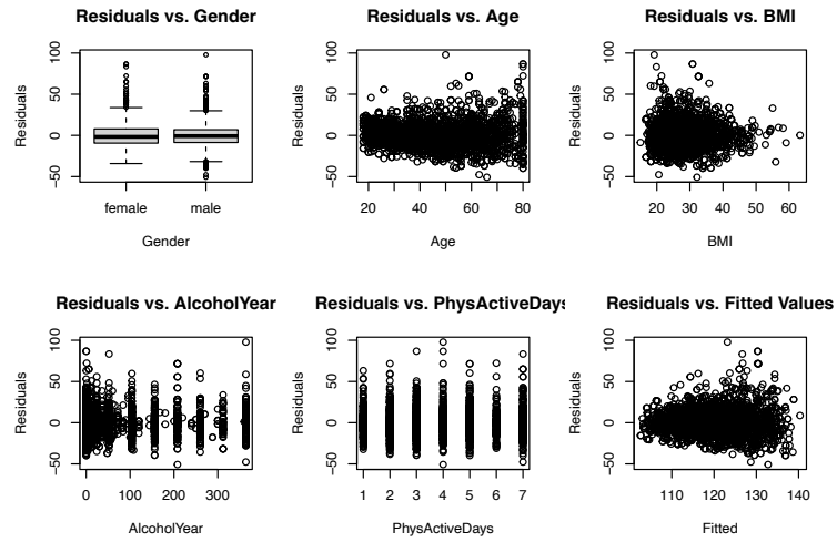
Figure 2: Residuals vs. Predictors in the preliminary model
