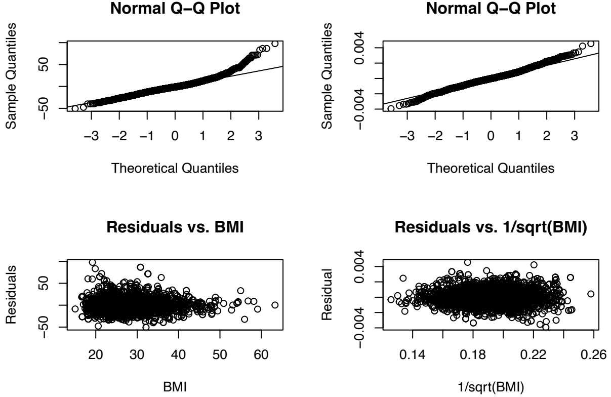
Figure 4: Before (left) and after (right) Box-Cox transformation, normality and constant variance improved
