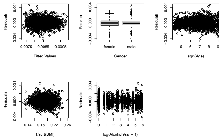
Figure 7: Residuals vs. predictors in the final model
