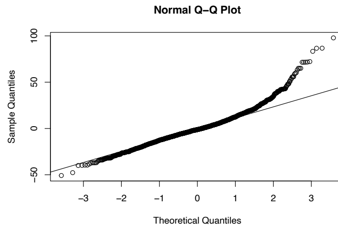
Figure 3: Q-Q plot for the preliminary model
